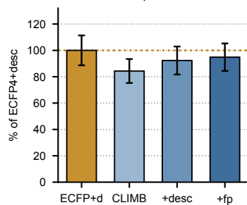
f Ames ↑
