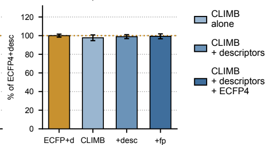
h QM7 ↓
