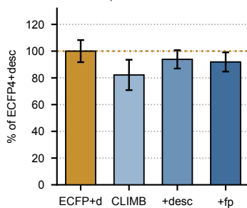
g Tox21 ↑
