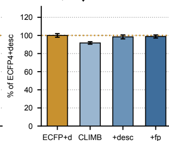
h QM7 ↓
