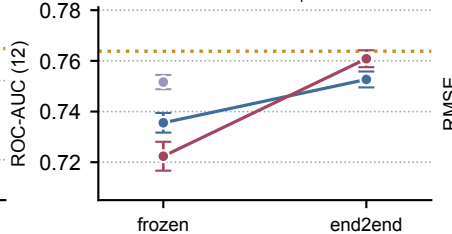
Tox21 ↑
