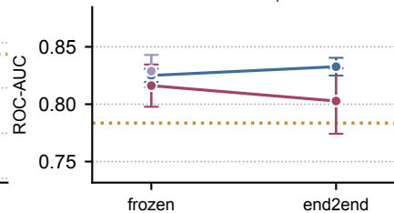
BACE ↑
