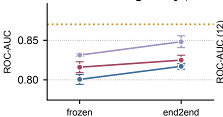
Ames Mutagenicity ↑
