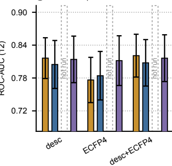
g Tox21 ↑
