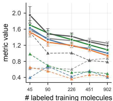
ESOL (RMSE ↓)
