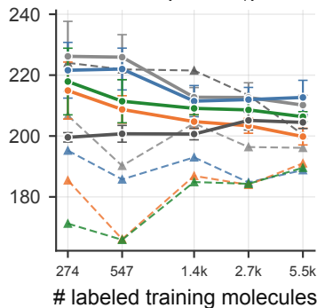
QM7 (RMSE ↓)
