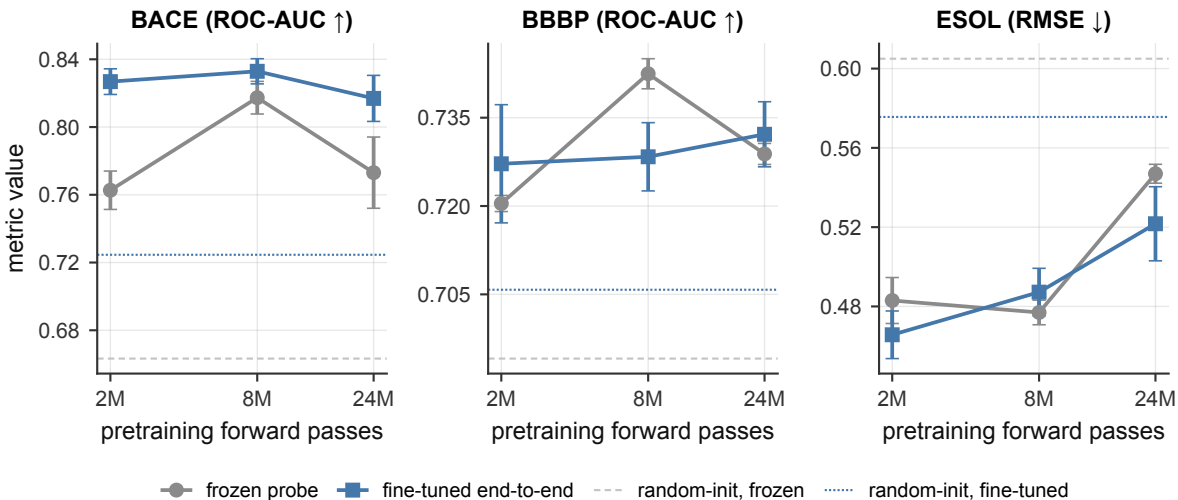
Fig E1 - is the flat pretraining ladder a frozen-probe artifact?
