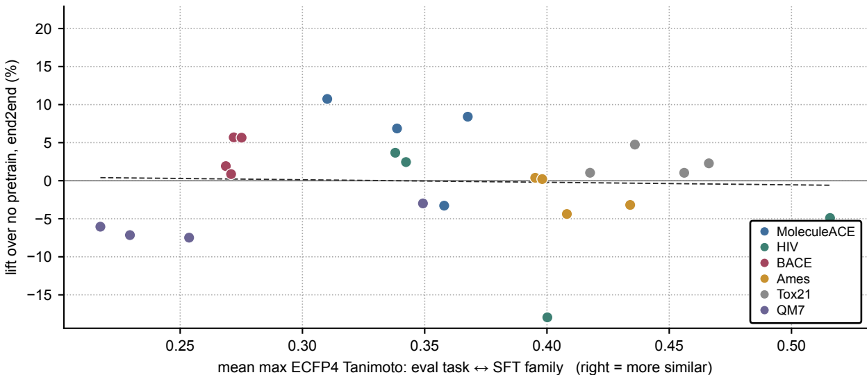
Fig C2 — Supervised pretraining: transfer vs chemical similarity (n=24, Pearson r=-0.04 , Spearman \rho=-0.01 , p=0.945 )
