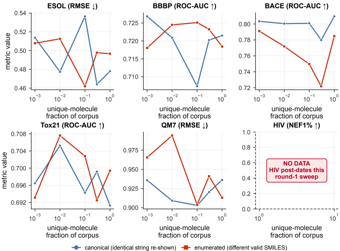
Fig H1 - does SMILES enumeration beat canonical repetition? (unsup_only)
