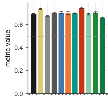
Tox21 (7,823 mols) (ROC-AUC ↑ · n_test = 784)
