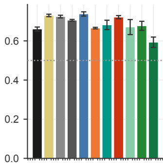
BBBP (2,039 mols) (ROC-AUC ↑ · n_test = 204)
