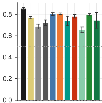
BACE (1,513 mols) (ROC-AUC ↑ · n_test = 152)
