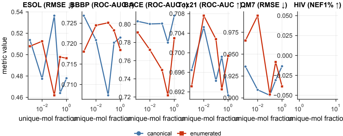
Fig H1 (H8) — canonical vs enumerated SMILES (unsup_only, downstream lift)
