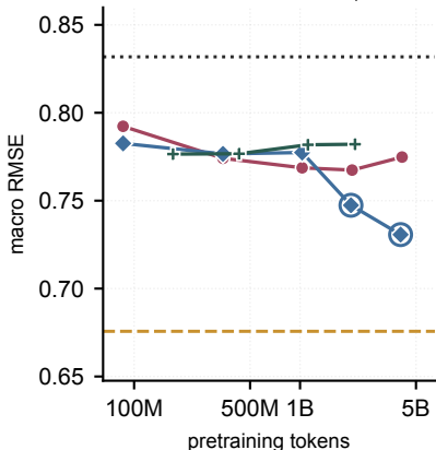
hERG ↑
