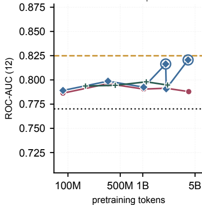
Tox21 ↑
