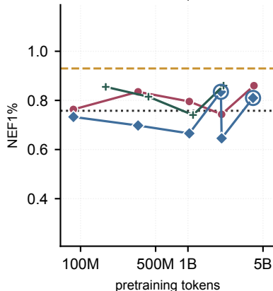
Tox21 ↑
