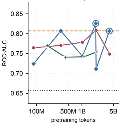
hERG ↑
