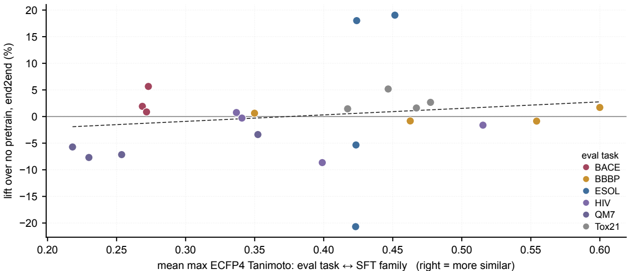
Fig C2 — Supervised pretraining: transfer vs chemical similarity (n=24, Pearson r=+0.16 , Spearman \rho=+0.22 , p=0.292 )
