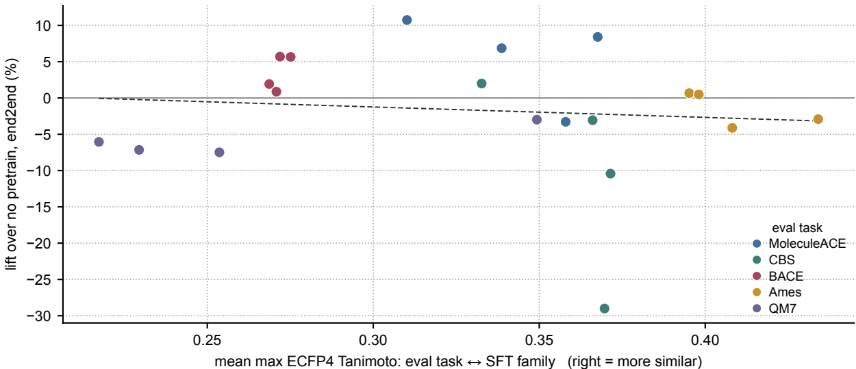
Fig C2 — Supervised pretraining: transfer vs chemical similarity (n=20, Pearson r=-0.11 , Spearman \rho=-0.09 , p=0.719 )
