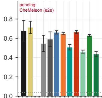
HIV (41,120 mols) (NEF1% ↑ · all scored, OOF)
