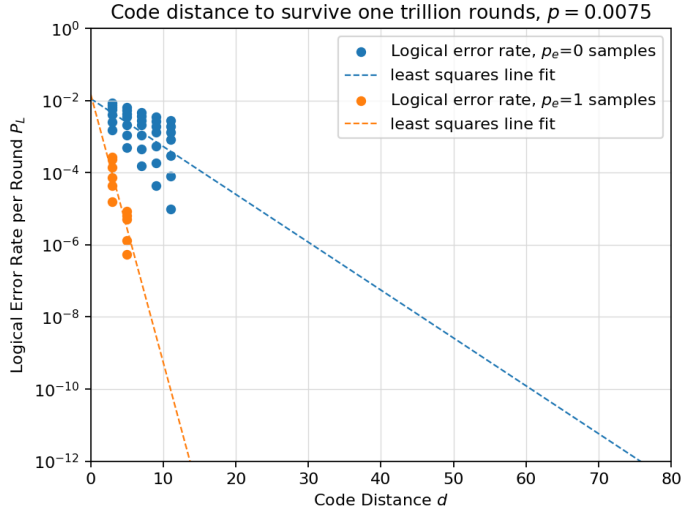
Figure 2: Among below-threshold ( p_{thr} = 0.0075 ) samples, the minimum code distance d \approx 15 is projected to survive one trillion rounds with full erasure conversion ( p_e = 1 ), an 80% decrease from d \approx 75 without erasure conversion ( p_e = 0 ).
