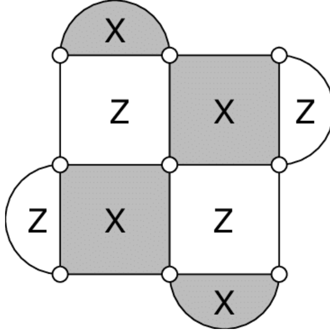
Figure 1: 9 Qubit Surface code.
