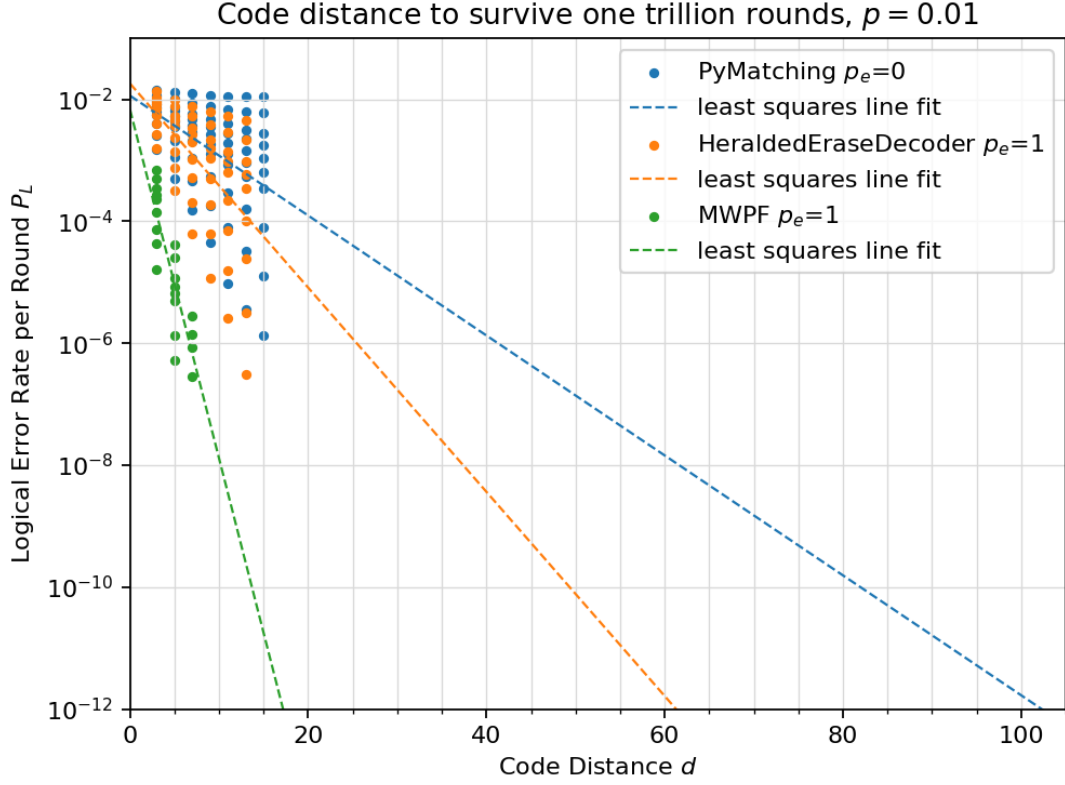
Figure 6: Among below-threshold ( p_{thr} = 0.01 ) samples, the minimum code distance d \approx 17 is projected to survive one trillion rounds with full erasure conversion ( p_e = 1 ) and Hypergraph MWPF syndrome decoding (green), and \approx 72\% decrease from d \approx 60 with erasure-aware edge re-weighting with MWPM (orange), and \approx 83\% decrease from d \approx 100 with MWPM in a pure Pauli noise regime with no erasures.
