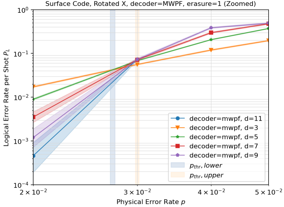
Figure 4: Circuit-level error threshold: hypergraph minimum-weight parity factor decoding for errors correlated to erasure events p_e . Comparison of logical error rate P_L with physical qubit error rate p converted to erasure errors. Following The lower and upper bounds of the threshold region p_{thr,s} between 2.70% and 3.02% is estimated from the d=3,5 and d=9,11 crossings. See: EXPERIMENT 3: ERASURE-AWARE MINIMUM-WEIGHT PARITY FACTOR .
