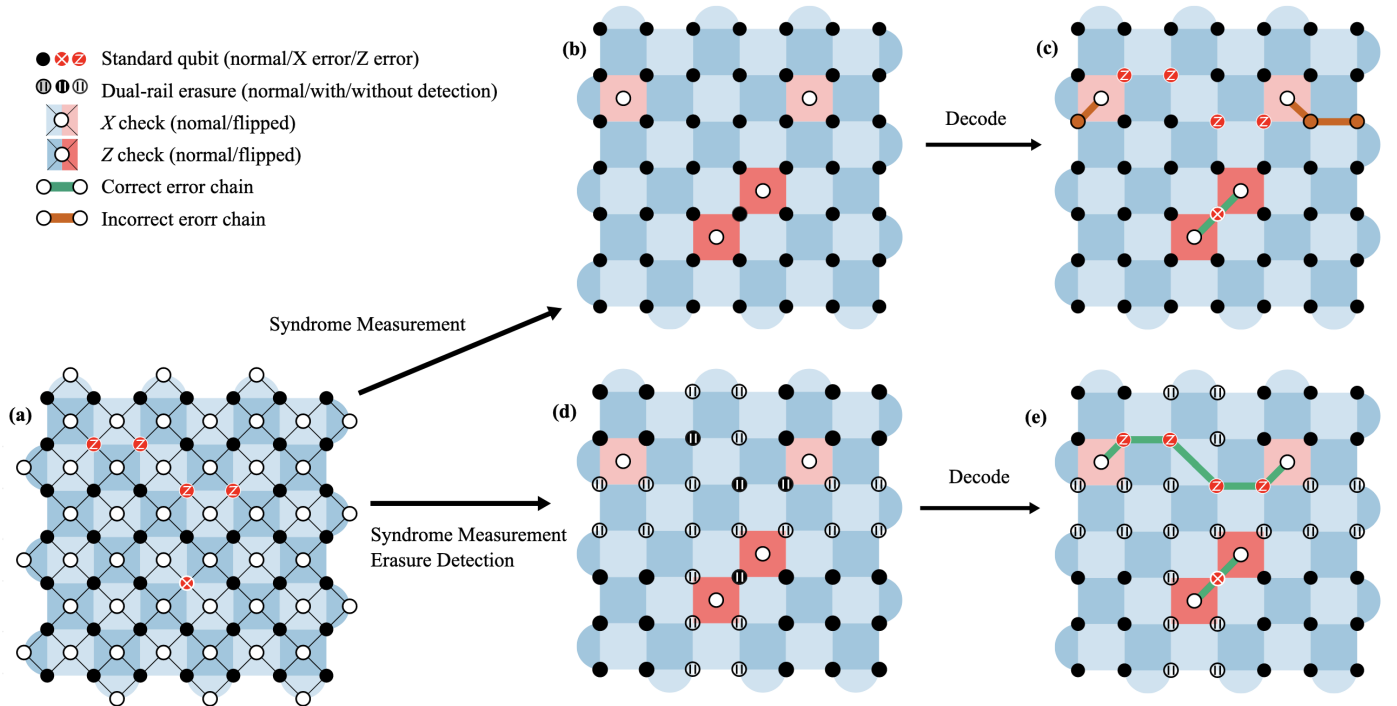
Figure 1: Dual-rail erasure-check qubits in superconducting transmons . (a) A set of errors occurring in the surface code. (b) Syndrome information available in a pure Pauli noise regime. (c) Decoder prediction that results in a logical Z error (orange path). (d) Syndrome information from parity-check ancilla qubits enriched with erasure checks. (e) A correlated erasure-aware error model weights the green path more heavily, avoiding the logical error in (b). [16]
