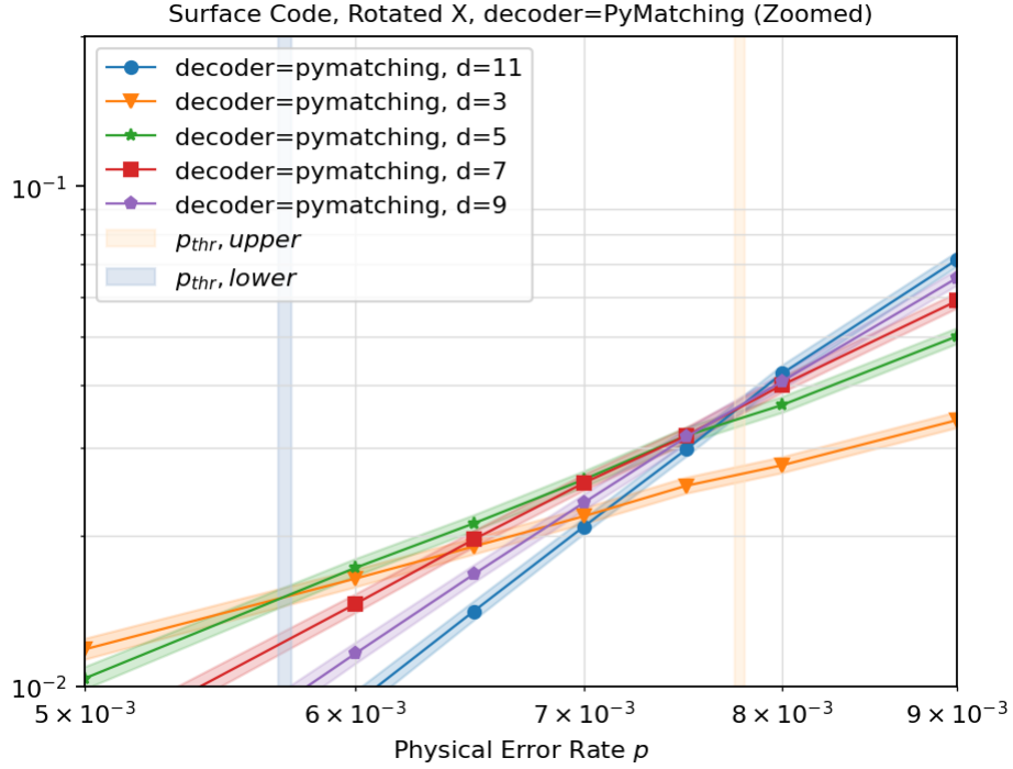
Figure 2: Baseline circuit-level error threshold: minimum-weight perfect matching. Comparison of logical error rate P_L with physical qubit error rate p modeled by uniform Pauli noise. The lower and upper bounds of the threshold region p_{thr} between 0.57% and 0.78% is estimated from the d=3,5 and d=9,11 crossings.
