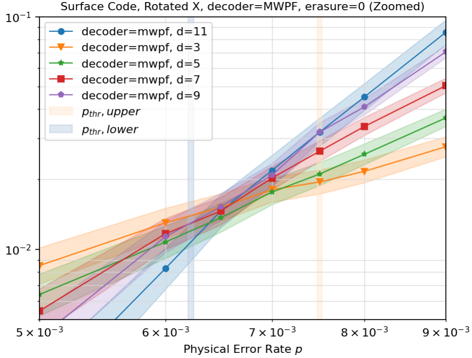
Figure 3: Baseline circuit-level error threshold: minimum-weight parity factor. Comparison of logical error rate P_L with physical qubit error rate p modeled by uniform Pauli noise. The lower and upper bounds of the threshold region p_{thrs} between 0.62% and 0.75% is estimated from the d=3,5 and d=9,11 crossings.
