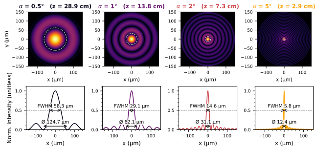
FIG. 8. TODO caption about axicon angle + radial core diameter.
