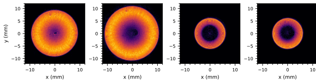
FIG. 14. TODO caption about axicon 1-2 alignment, annu- lus quality, and on-axis intensity ripples.
