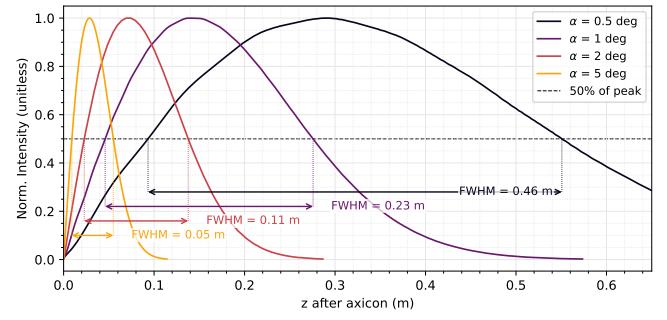
FIG. 9. TODO caption about axicon angle + bessell zone length.
