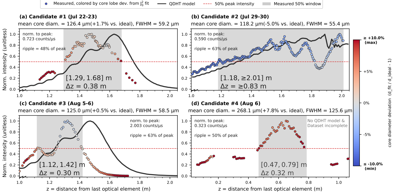
FIG. 6. Measured on-axis intensity I(0, z) along the propagation direction for candidates (a) #1, (b) #2, (c) #3, and (d) #4 in Table I. Each panel normalized to its own peak intensity rate (counts/μs). z is measured from the last optical element. Points are J_0^2 amplitudes fit to cropped cross-section images of the plane transverse to the propagation direction. Points are colored by the deviation of the fitted central/core lobe diameter from the ideal value. The solid black line is the QDHT model, dashed red line indicates 50% of the measured peak, and the grey shaded region is the measured Bessel zone Z_R between the outermost 50% crossings. The ripple metric is the peak-to-peak variation of the on-axis intensity within the measured Bessel zone. Candidate #2's Bessel zone was not fully characterized due to space limitations on the optics table, so the measured Z_R and \Delta Z_R should be interpreted as lower bounds. No QDHT model was developed for candidate #4, which placed a 2× magnification telescope inside the Bessel zone.
