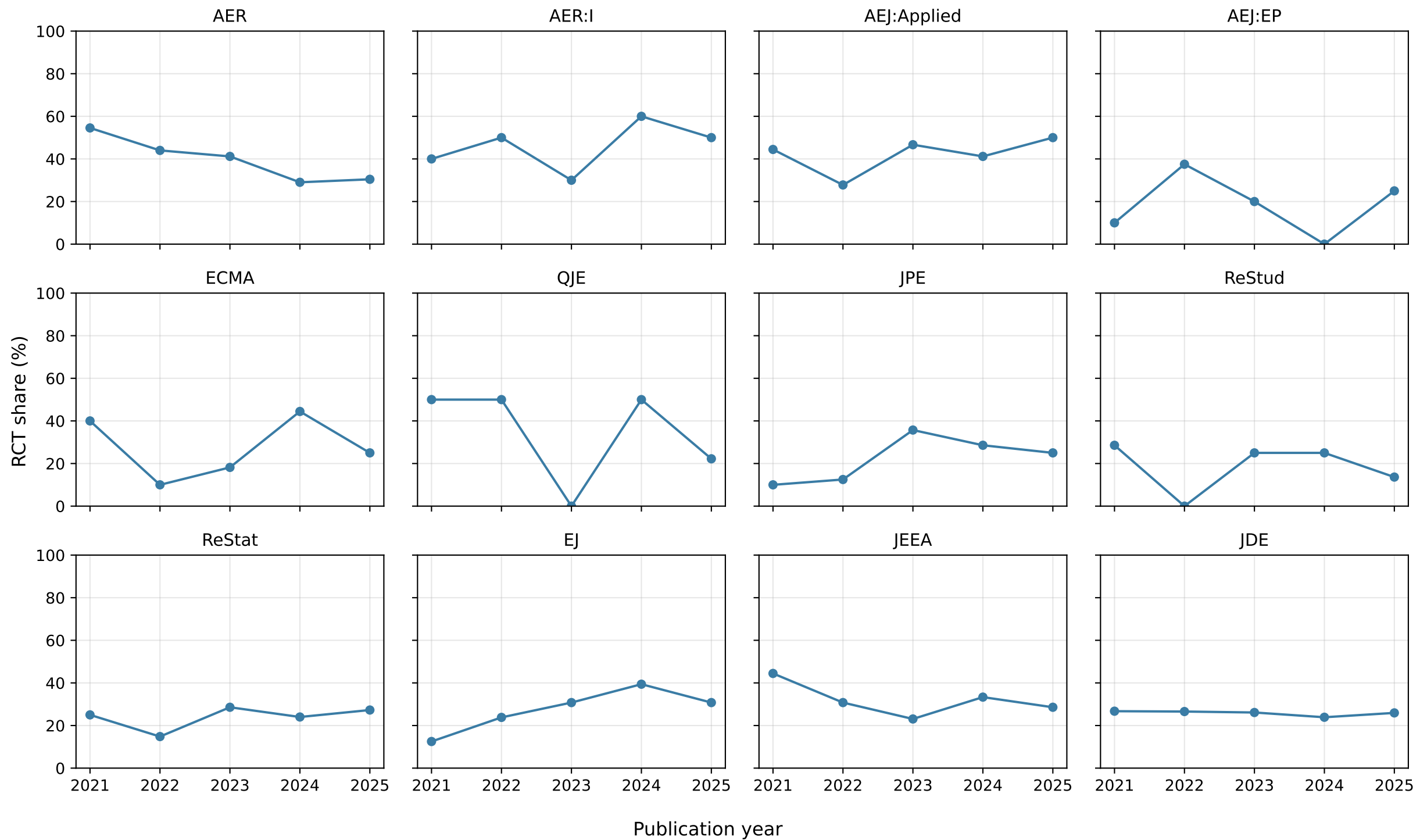
RCT share by journal × year, 2021-2025
