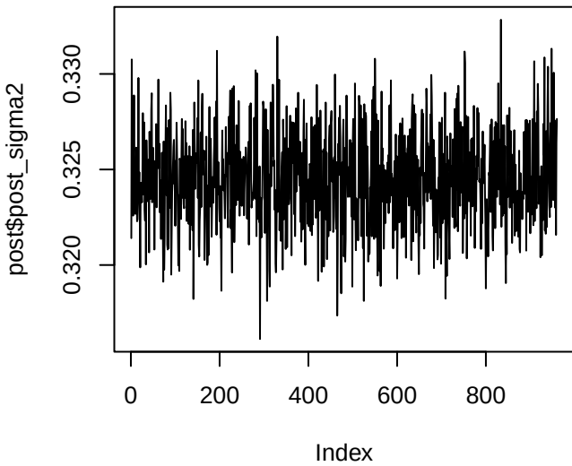
Trace of \sigma^2
