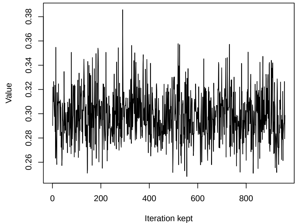
Post-burn-in trace of \tau
