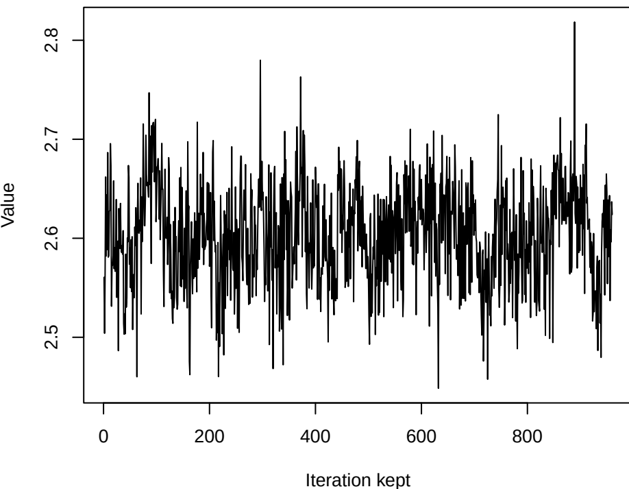
Post-burn-in trace of \sigma^2
