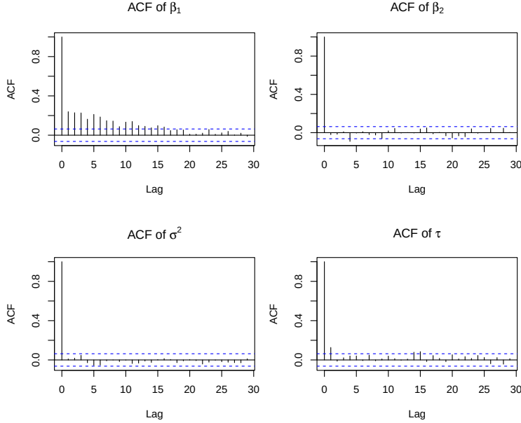
Figure 4: Post-burn-in autocorrelation functions for selected model parameters.
