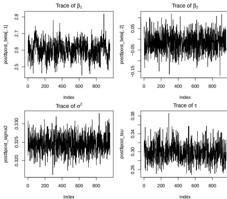
Figure 3: Post-burn-in trace plots for selected model parameters.
