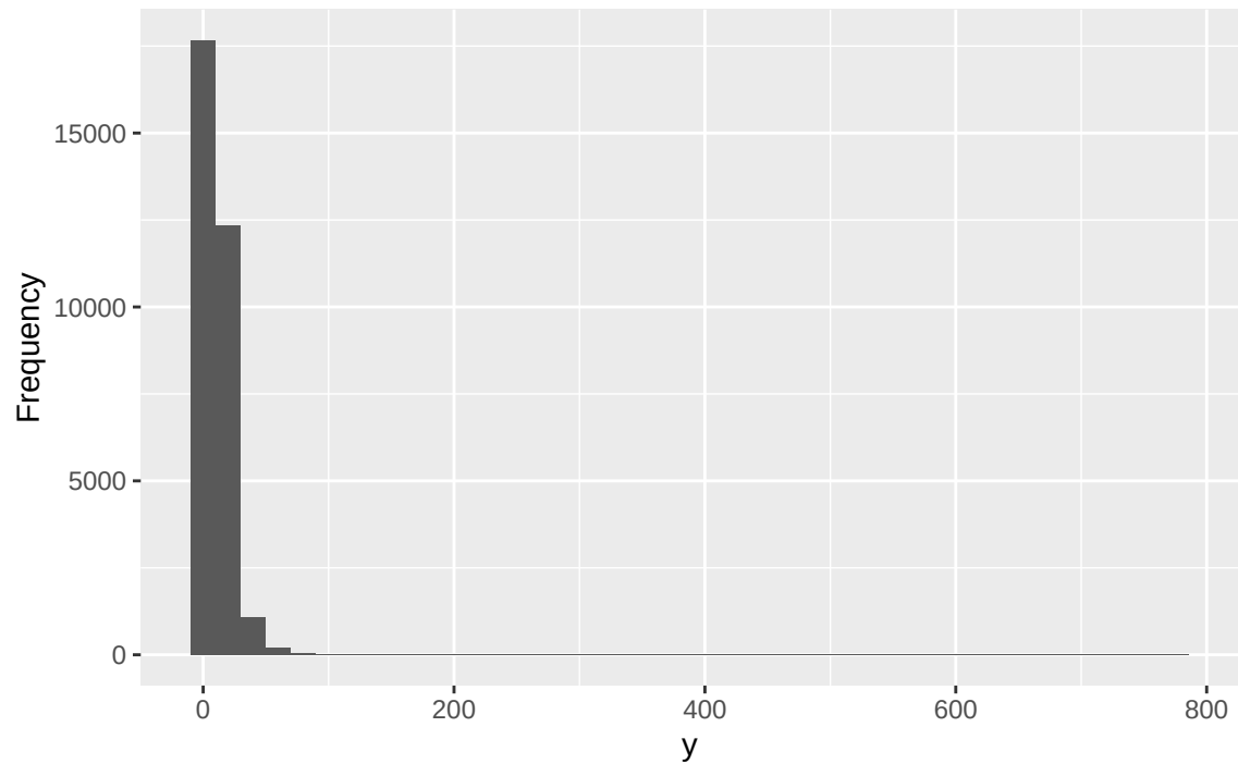
Distribution of the raw PM2.5 outcome
