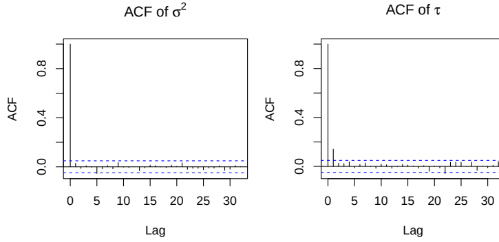
Figure 4: Post-burn-in autocorrelation functions for the variance components.
