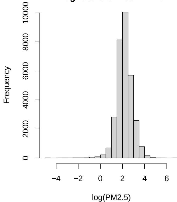
Log-transformed PM2.5
