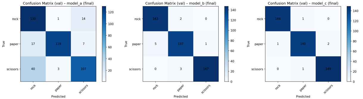
Figure 3: Validation confusion matrices for the three final architectures (models A–C).
