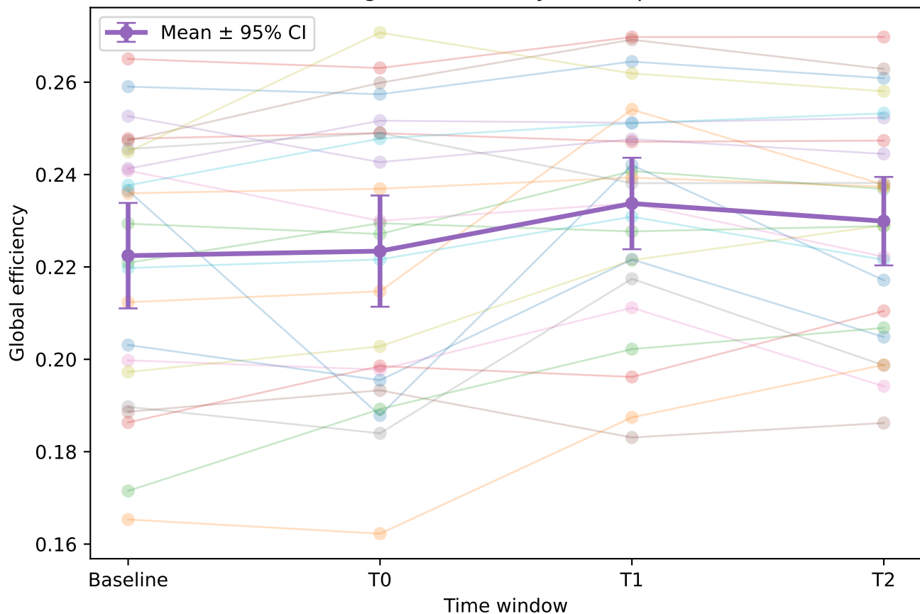
Delta coherence global efficiency across peri-ictal windows
