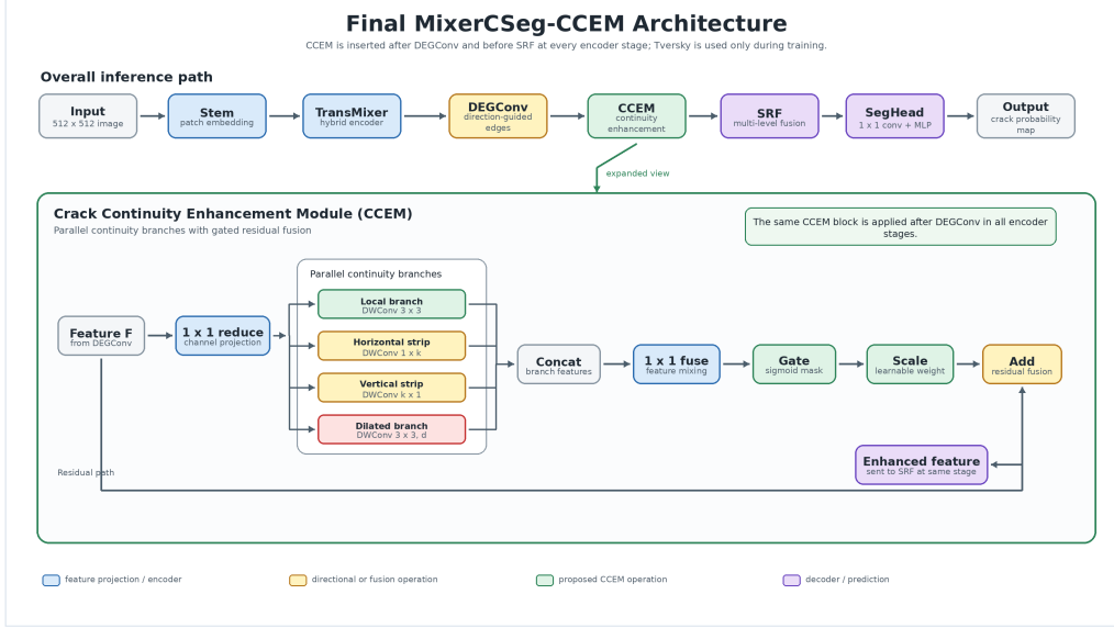
Figure 1: Overall architecture of the final method. CCEM is inserted after DEGConv at all encoder stages while the original MixerCSeg data pipeline and decoder are kept unchanged.
