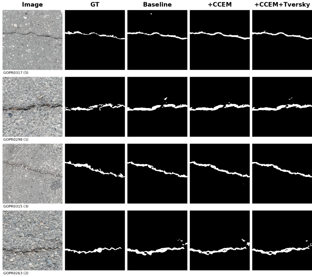
Figure 2: Qualitative comparison on CrackMap. Predictions are binarized using each method’s ODS threshold.
