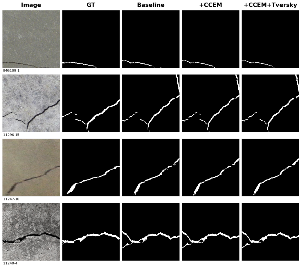
Figure 3: Qualitative comparison on DeepCrack. Predictions are binarized using each method’s ODS threshold.
