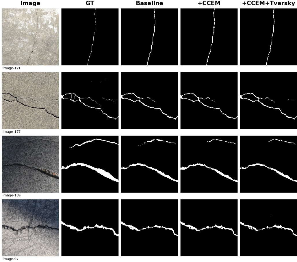
Figure 4: Qualitative comparison on CamCrack789. Predictions are binarized using each method’s ODS threshold.
