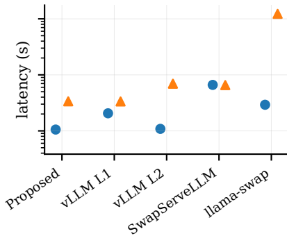
qwen-1.5b
