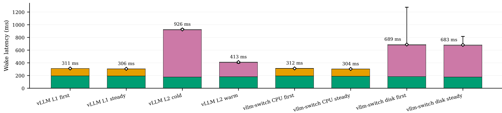
(b) Wake Latency Profiling
