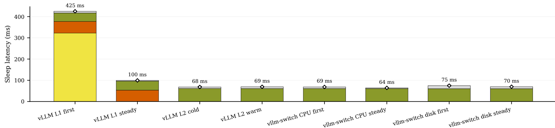
(a) Sleep Latency Profiling
