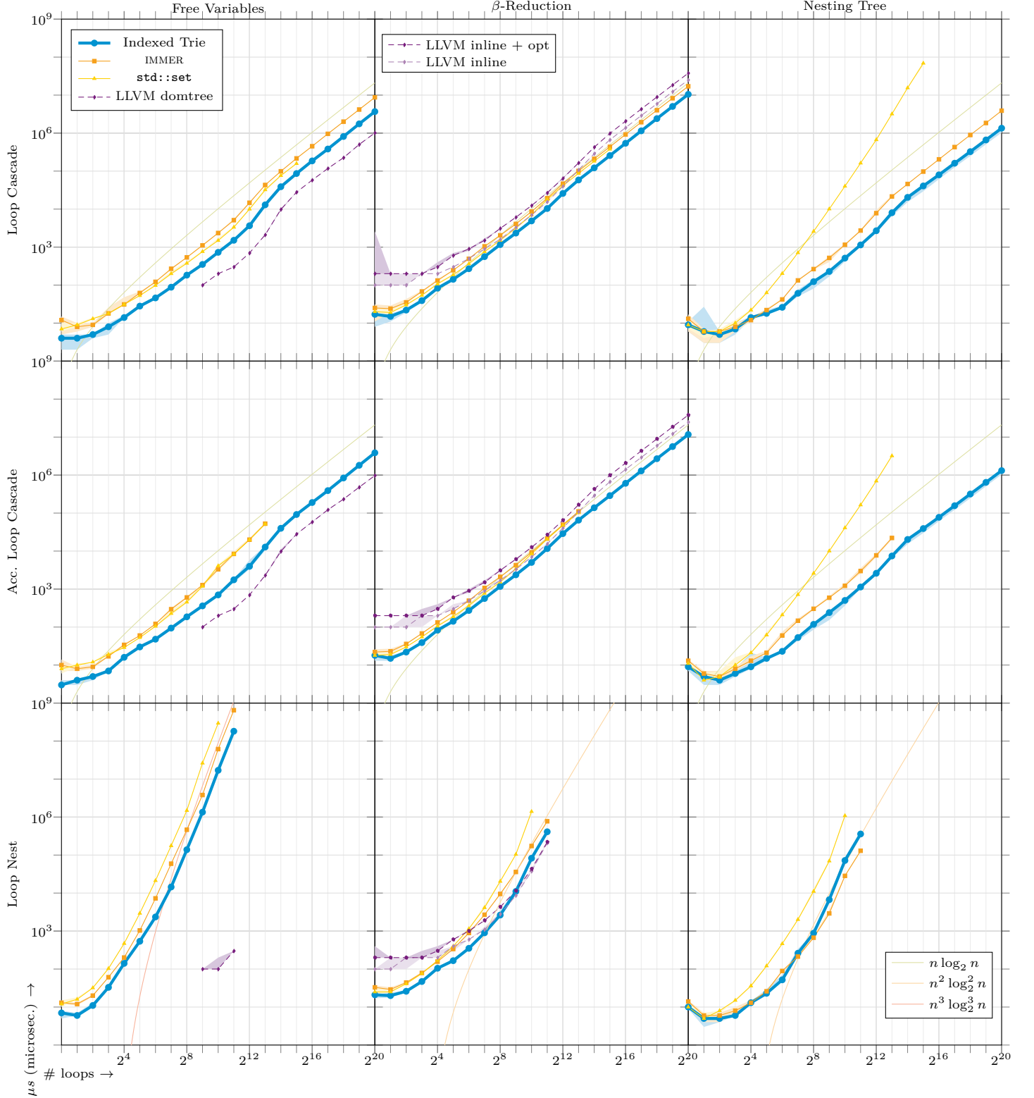
Figure 1: Performance (in \mu\text{s} , lower is better) of three operations—free variable computation, \beta -reduction, and nesting tree computation—on three synthetic programs with increasing numbers of loops. The plots compare three different set implementations: the indexed trie, IMMER, and std::set . Additionally, free variable computation is compared against LLVM’s dominance analysis; \beta -reduction is compared against LLVM’s inliner, both with and without optimizations that simulate MIMIR’s on-the-fly optimizations. For reference, 10^3 \mu\text{s} = 1 \text{ ms} , 10^6 \mu\text{s} = 1 \text{ s} .
