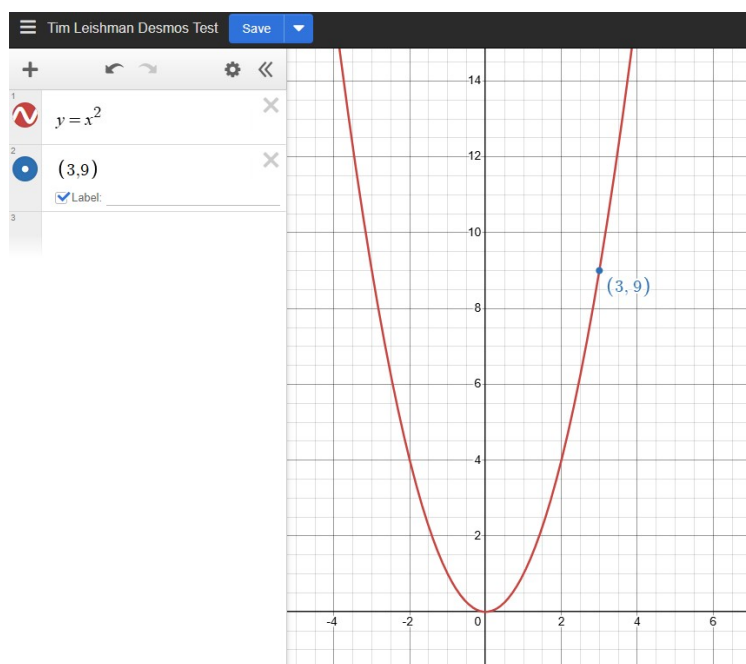
Figure 1.6: y = x^2
