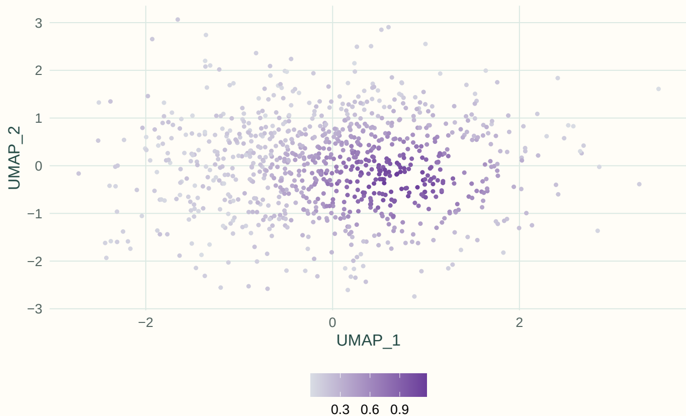
Feature plot: marker intensity on embedding
