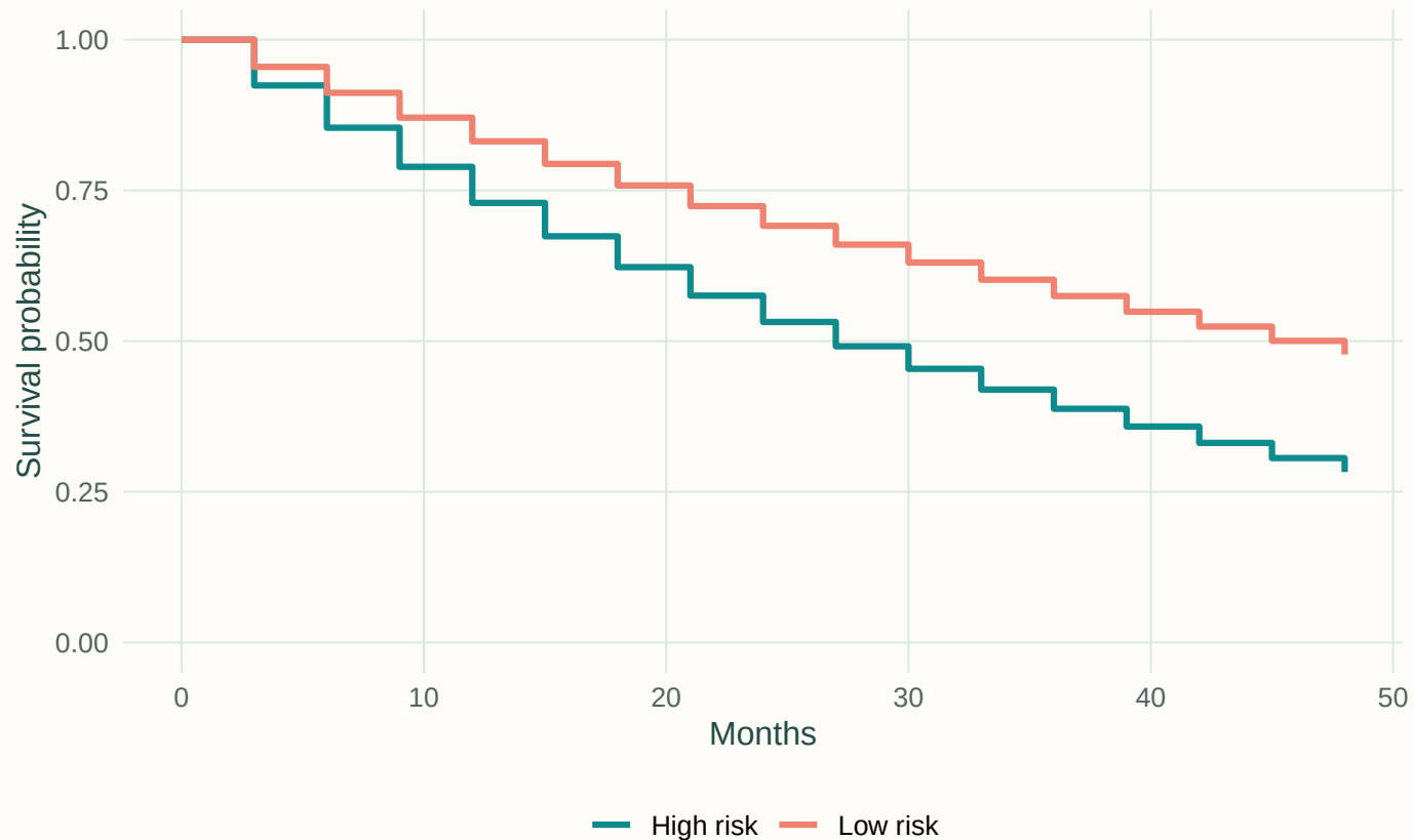
Kaplan–Meier curve: survival by risk group
