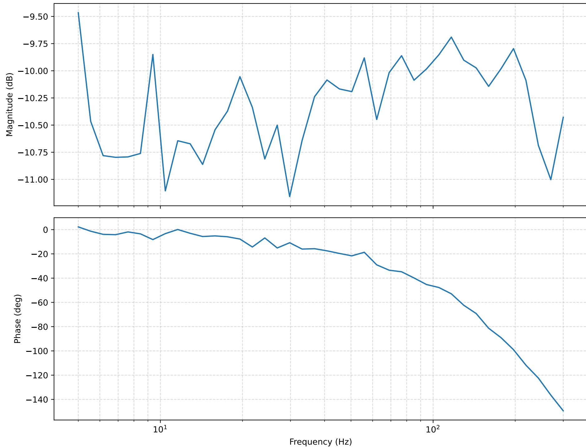
Bode Plot
