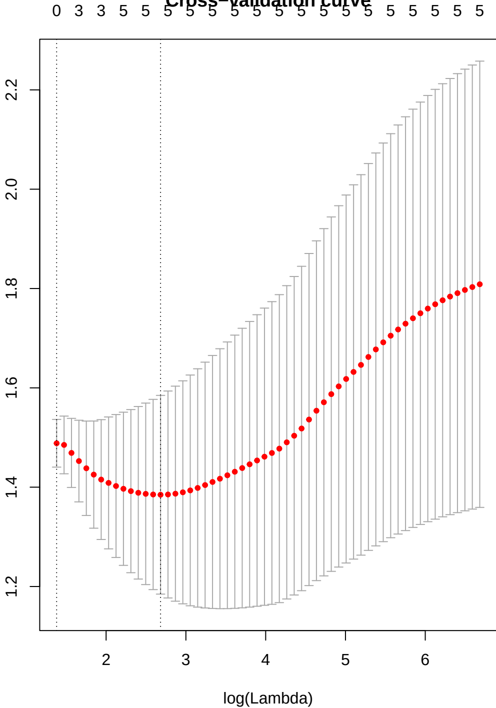
Cross-validation curve
