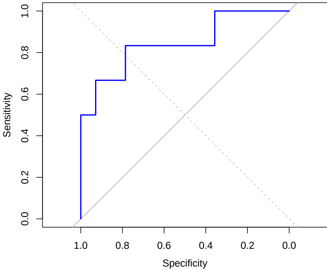
Training Set ROC Curve (AUC = 0.845)
