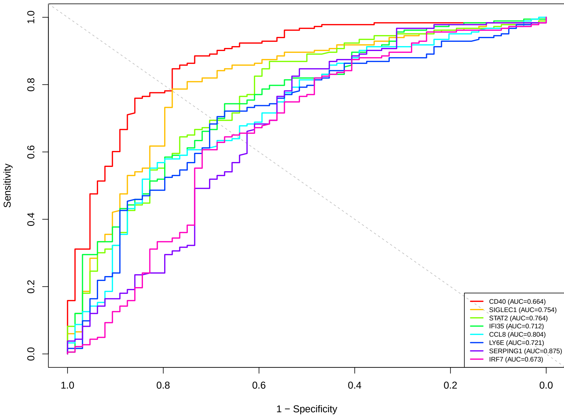
Top Single Gene ROC Curves
