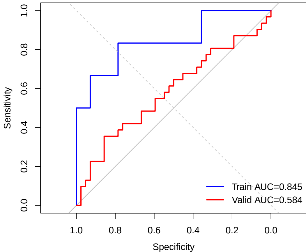
ROC Curves: Training vs Validation
