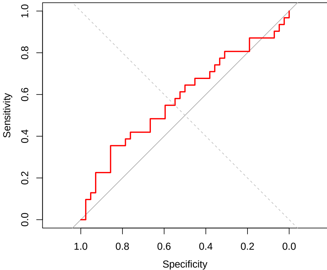
Validation Set ROC Curve (AUC = 0.584)
