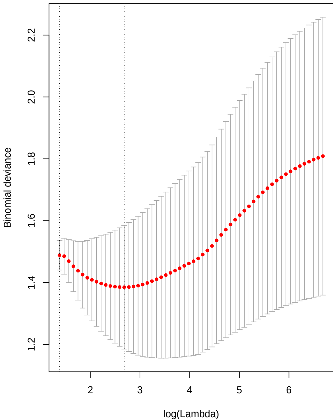
Cross-validation curve
