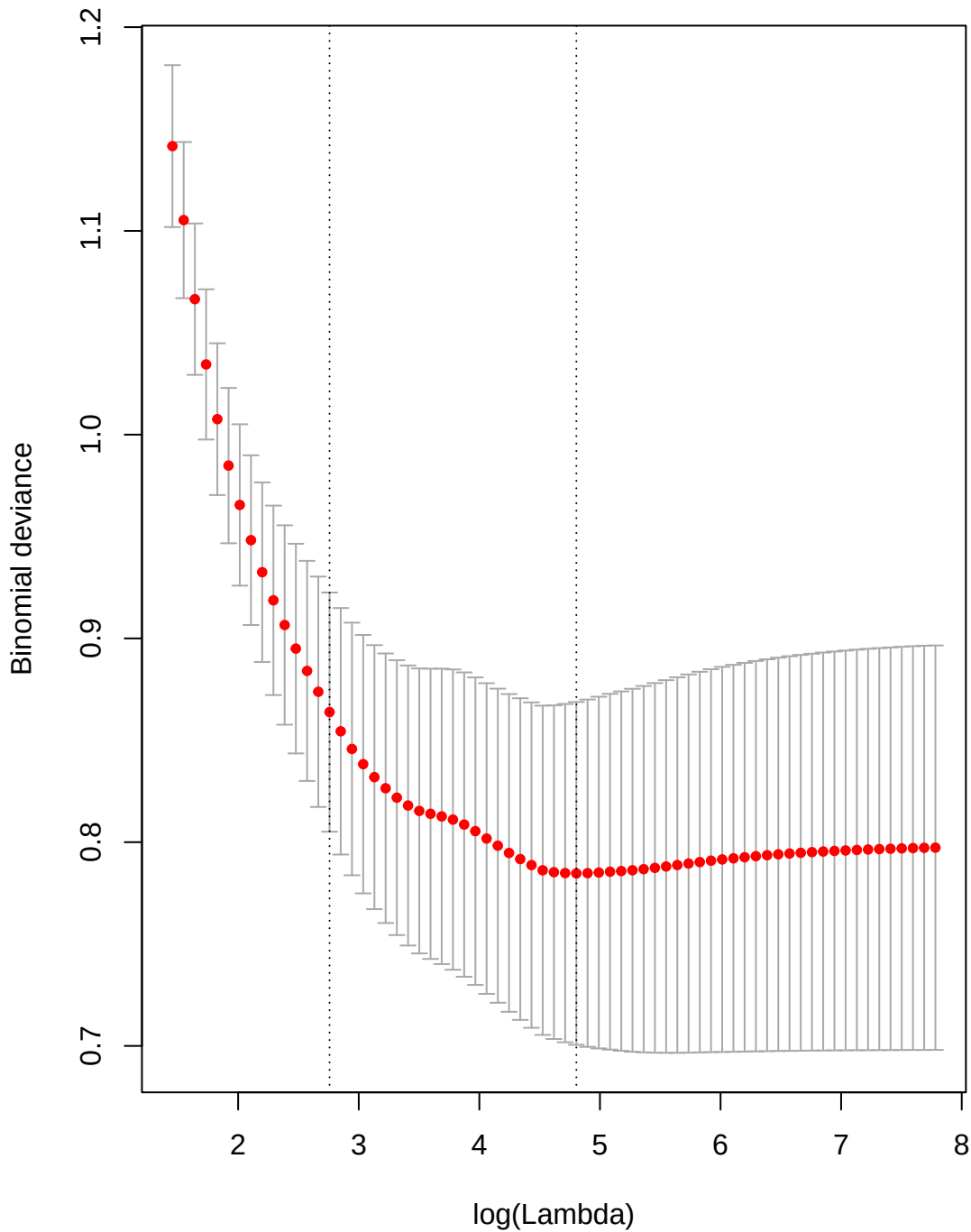
Cross-validation curve
