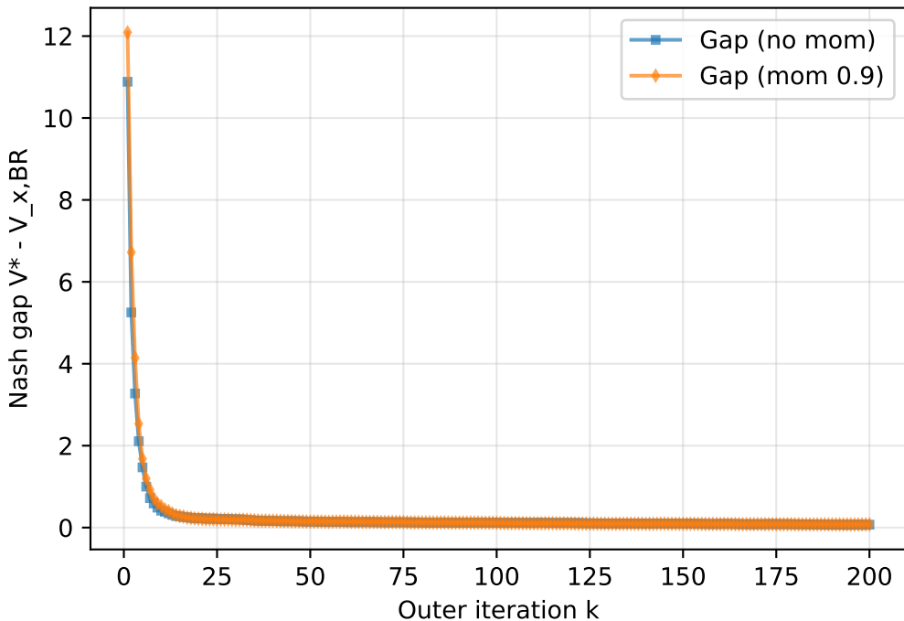
Distance to Nash (no-mom vs mom)
