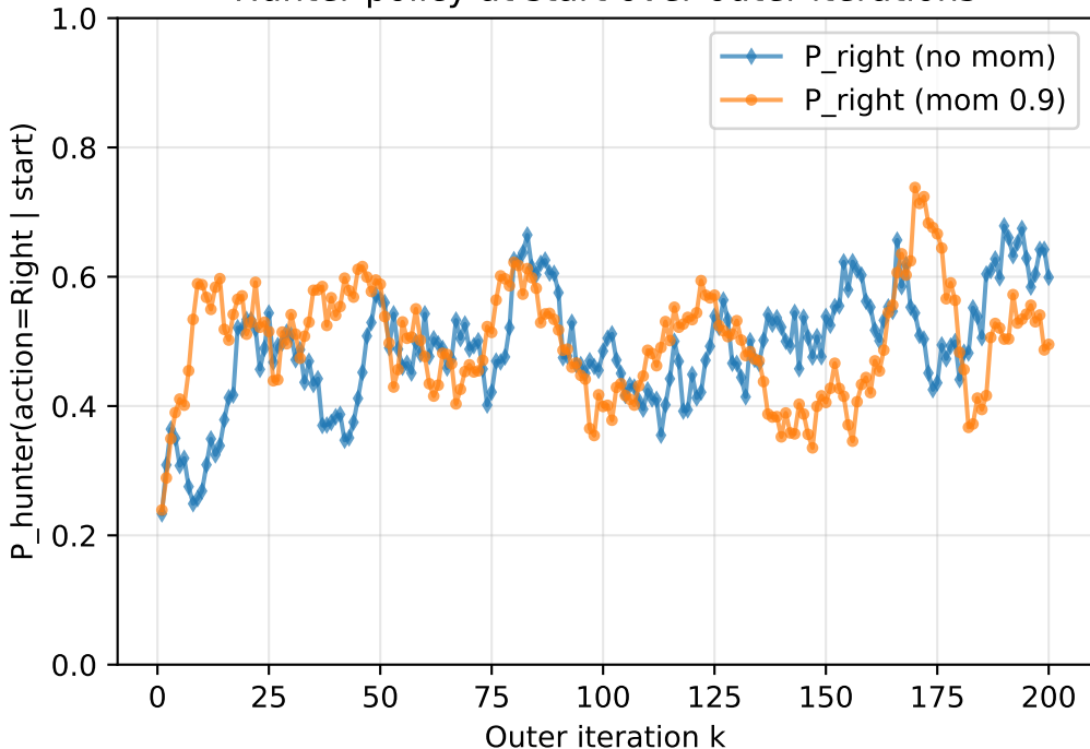
Hunter policy at start over outer iterations
