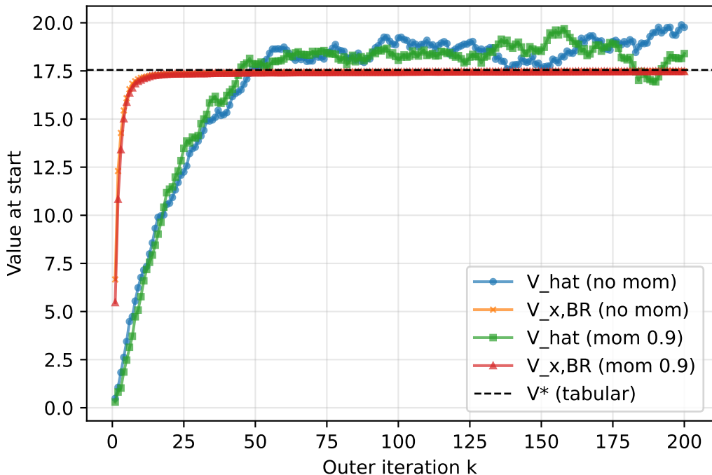
Approx vs True vs Best-Response Value (no-mom vs mom)
