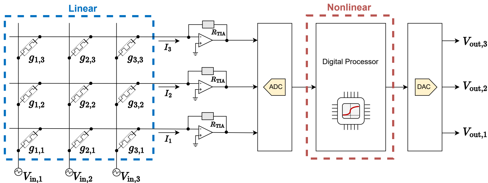
Hardware Implementation
