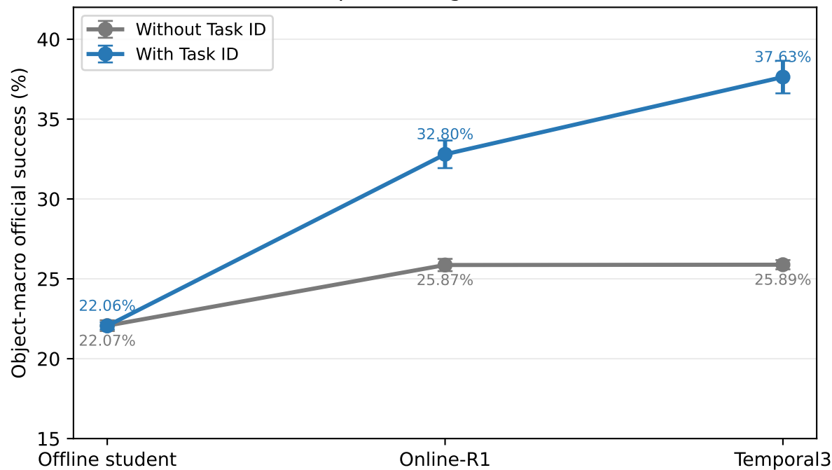
Pipeline-stage success
