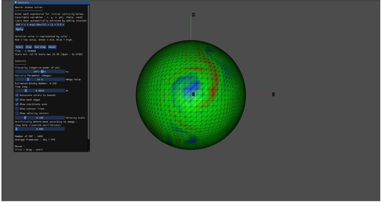
Figure 8: Top view (along the z -axis) of the vorticity field at t \approx 2 days. The flow is dominated by coherent large-scale vortices, characteristic of quasi-geostrophic dynamics.
