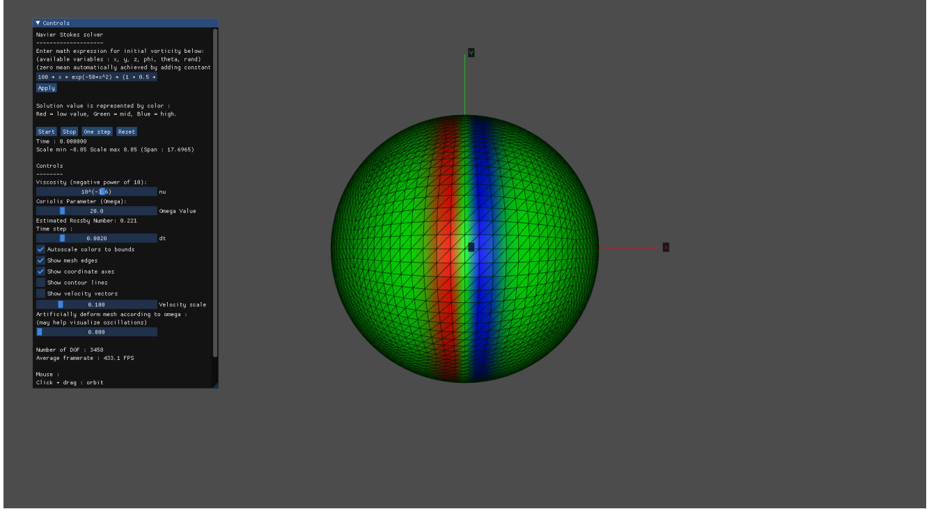
Figure 5: Initial state ( t = 0 ). The vorticity is concentrated in a narrow longitudinal band.
