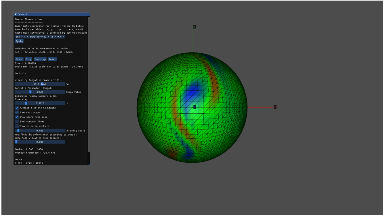
Figure 6: Snapshot at t \approx 1 . The initial vorticity bands have destabilized and reorganized into coherent structures driven by the strong planetary rotation.
