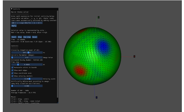
Figure 4: t \approx 13.1 : Final state showing stable, laminar decay.
