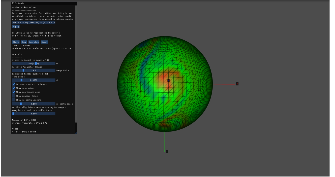
Figure 9: Bottom view (along the -z -axis) of the vorticity field at t \approx 2 days.
