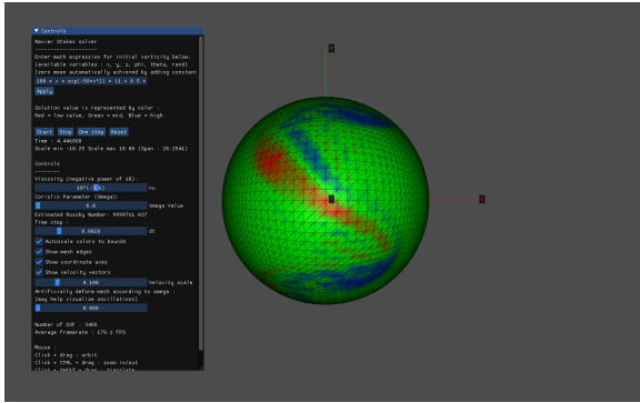
Figure 3: t \approx 4.4 : Initial band diffusion and lack of latitudinal migration.
