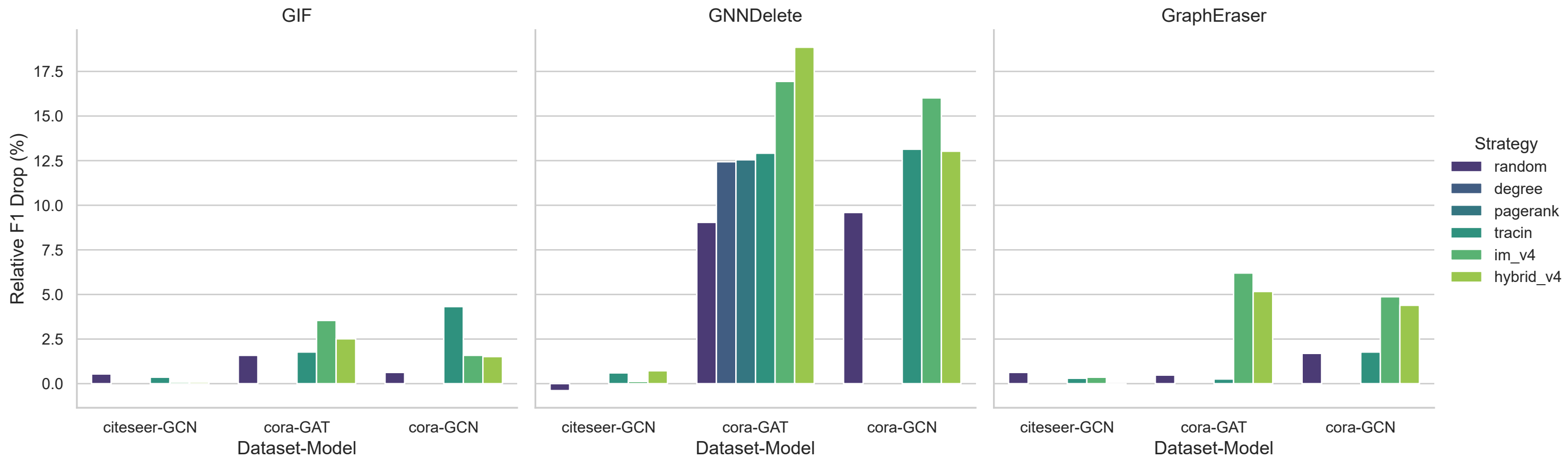
FIG-1: Generalization Potency (Relative F1 Drop vs. Random k=5 Baseline)
