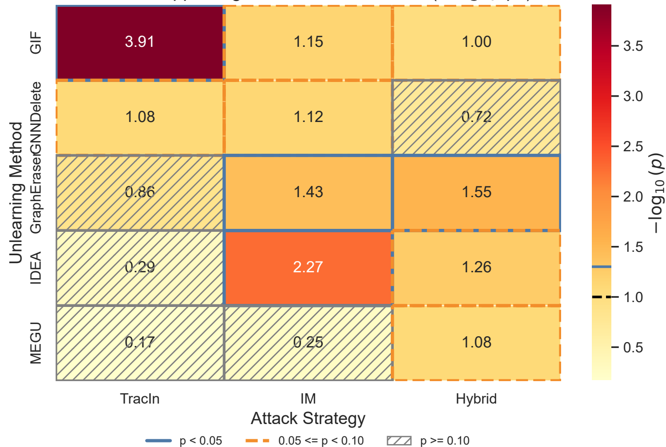
FIG-4a: Support Against Random Deletion ( -\log_{10}(p) )
