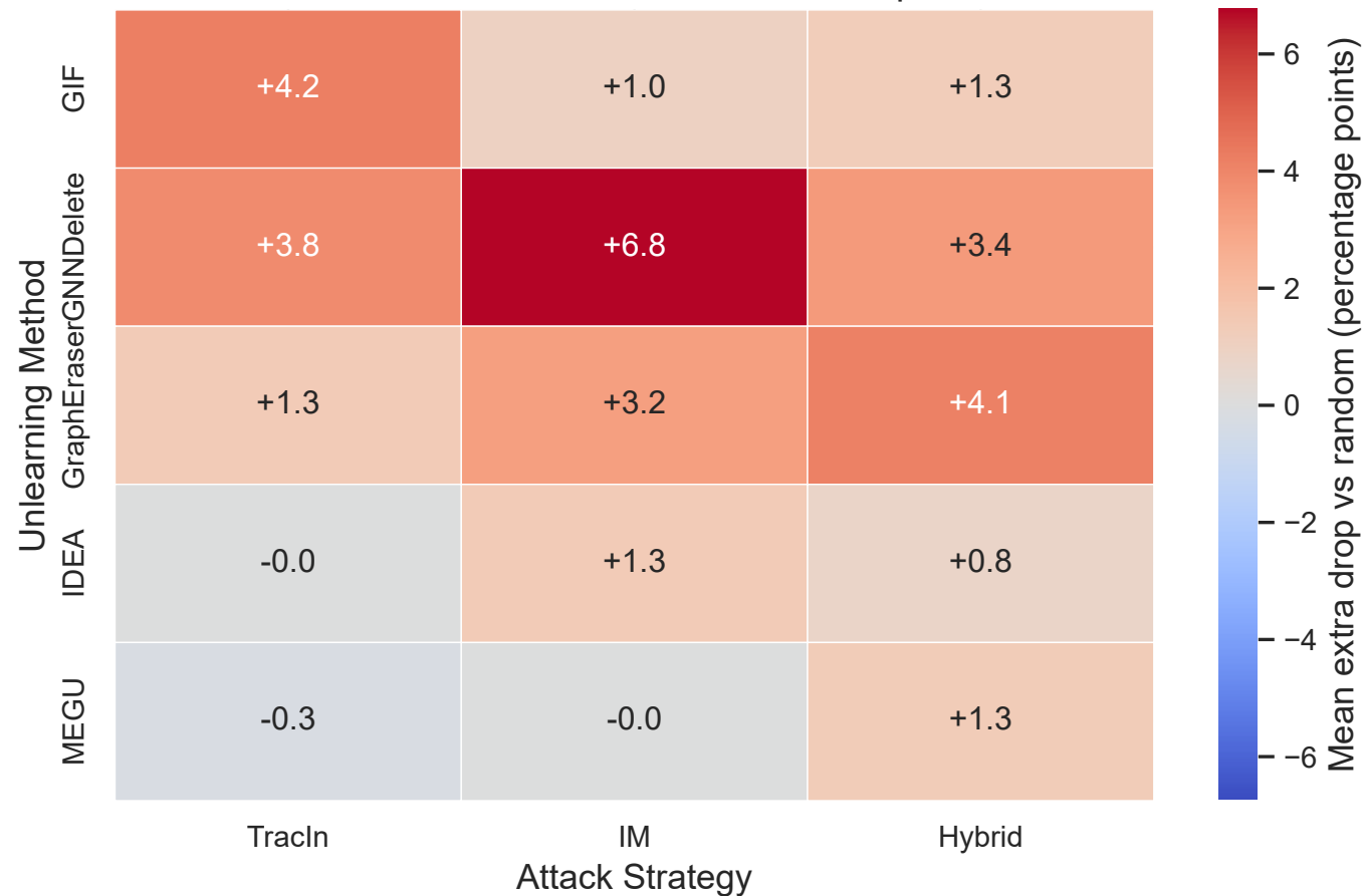
FIG-4b: Effect Size Against Random Deletion Cell values show mean extra relative F1 drop vs random
