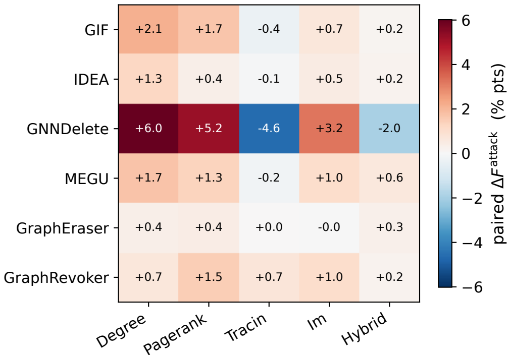
Effect size vs. random (Cora/GCN)
