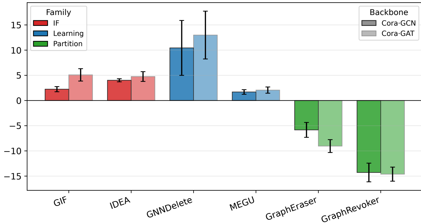
Architectural F1 shift at attack budget (negative = Shard Protection)
